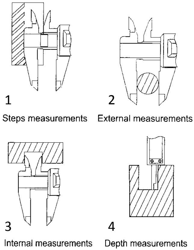
Figure 12-8 a & b illustrate four ways a caliper can be used to take measurements.
